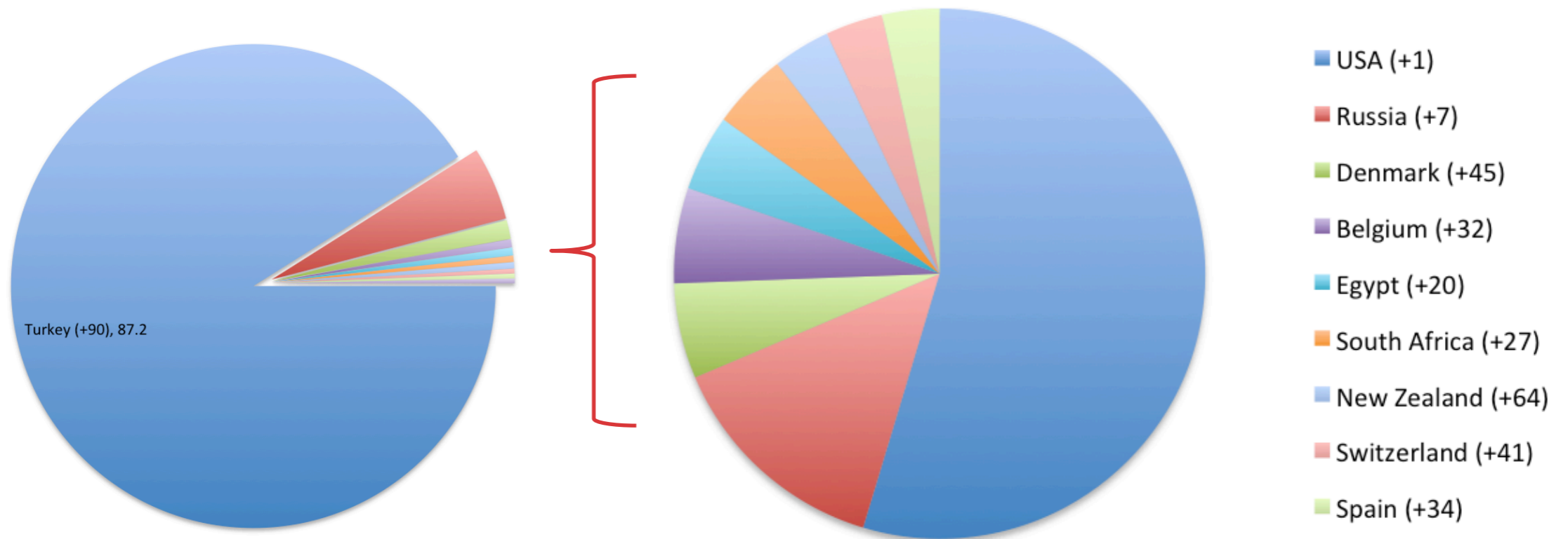
NXDOMAIN results
